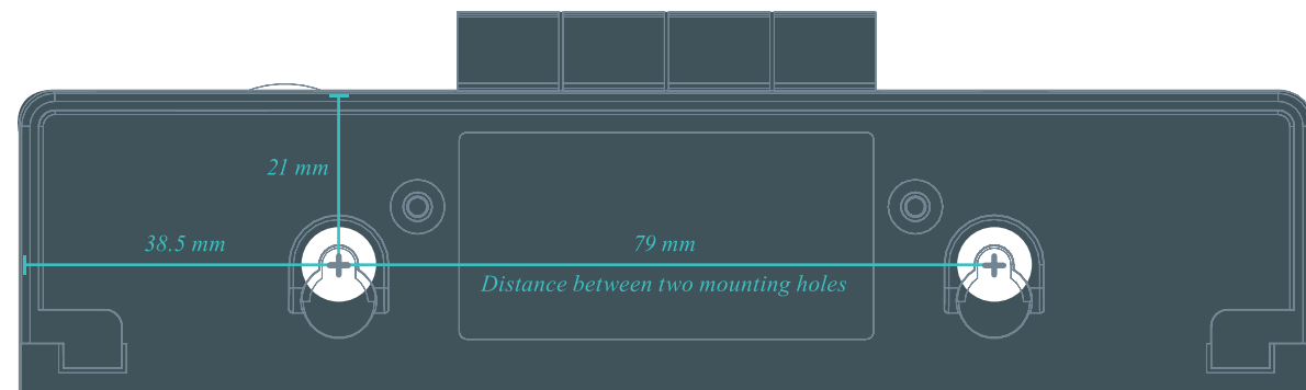
1:1 SCALE MOUNTING TEMPLATE FOR WALL SCREWS
