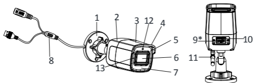
Figure 1-3 Overview of Type II
