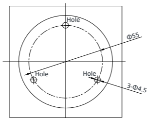
Figure 2-4 Drill the Holes
