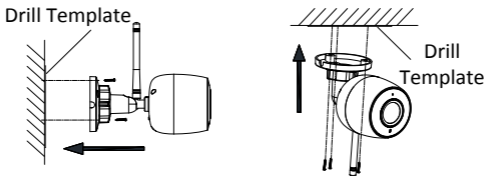
Figure 2-5 Install the Camera
