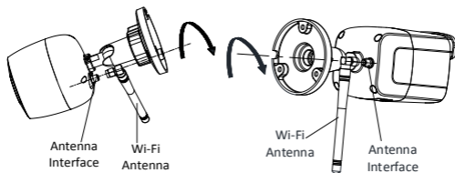
Figure 2-1 Mount the Antenna
