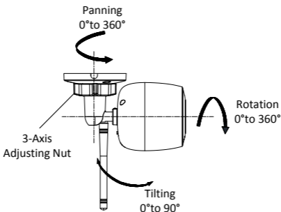
Figure 2-6 View Angle Adjustment
