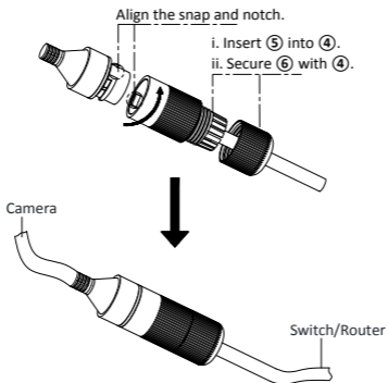
Figure 2-8 Waterproof Accessory Installation
