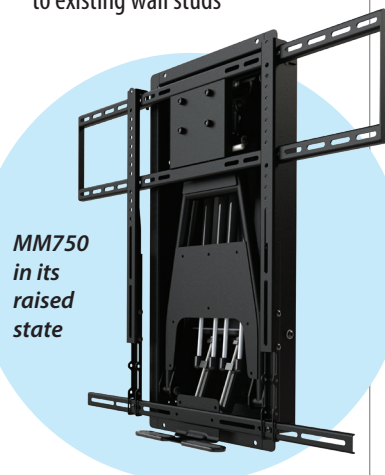
The MM750 comes with the Lifting Arm attached to the Housing/Recess Box
