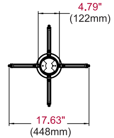
ADAPTOR PLATE
