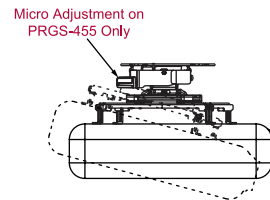
+15/- 20° PITCH
