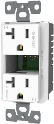
20A, 125VAC 5VDC, 2.0A NEMA 5-20R
