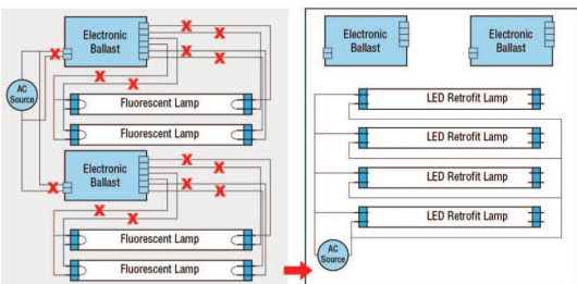
Figure 6. - Retrofit with Three/Four Lamps & Two Ballasts
