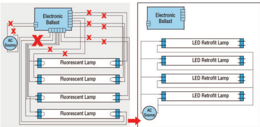
Figure 5. - Retrofit with Three/Four Lamps
