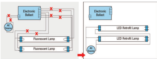
Figure 4. - Retrofit with Two Lamps
